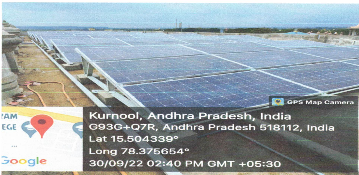
Clip-2: Solar Power Generating system -250kWp : Model- SL250KV6173-P2/Solarelectric 250kWp is under installation process shipped from Orb Energy Private Limited -Bangalore
